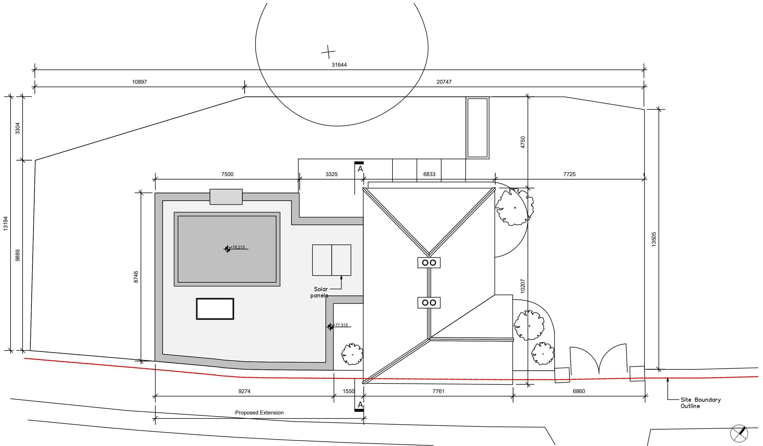
Gate Lodge, Proposed Roof Plans
